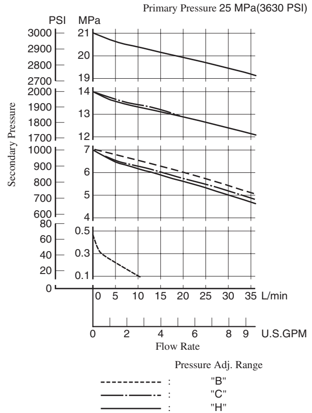
Nominal Override Characteristics
