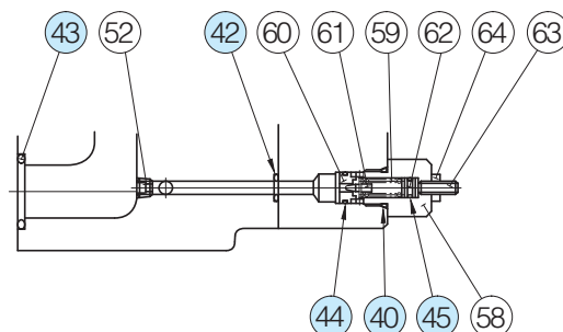
Section X-X
