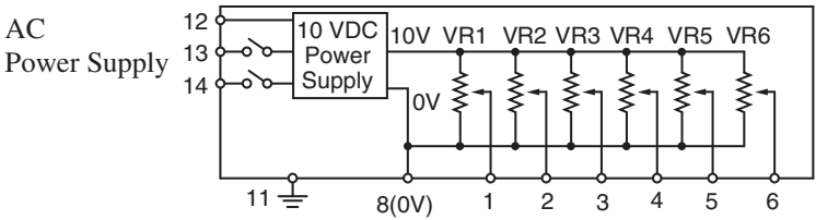
[Electric Circuit]
