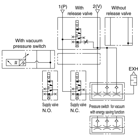
Circuit diagram
