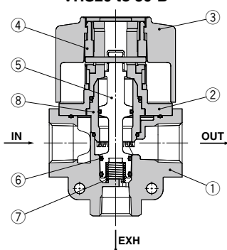
Cross section of EXH port
