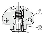
Cross section of EXH port
