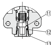
Cross section of EXH port
