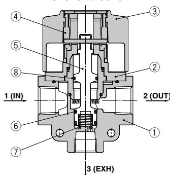
VHS2510 to 5510-B
