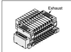
Direct EXH outlet with built-in silencer [-S]
