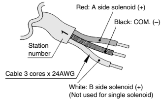
Single solenoid
