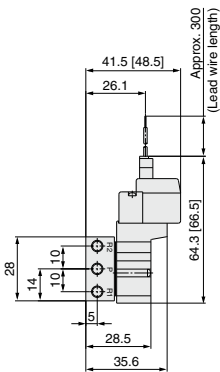
L plug connector (L): SYJ3140-□L□□-M5
