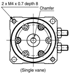
(Single vane)
