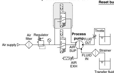
Air pilot actuation reset circuit
