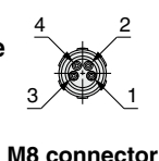
M8 connector
