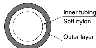
Sectional view of FR 2-layer tubing
