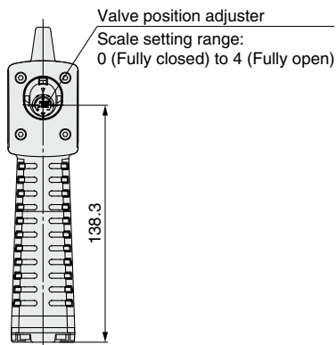
With adjuster
