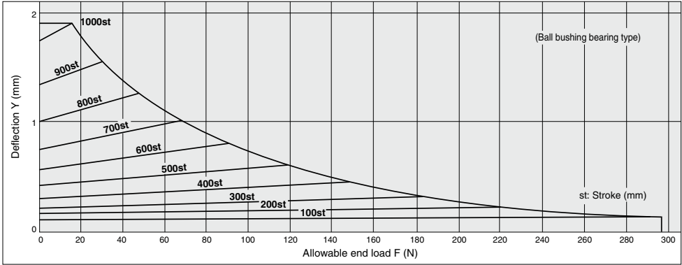
MGGL 100-Stroke
