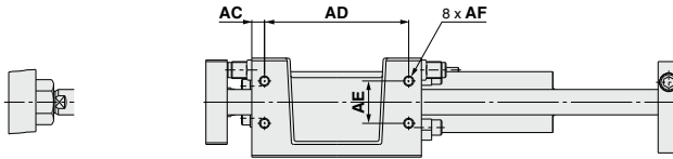
\phi 100 piston rod end connection
