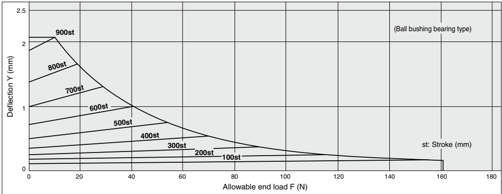
MGGL 63-Stroke
