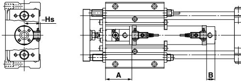
Auto Switch Mounting Height
