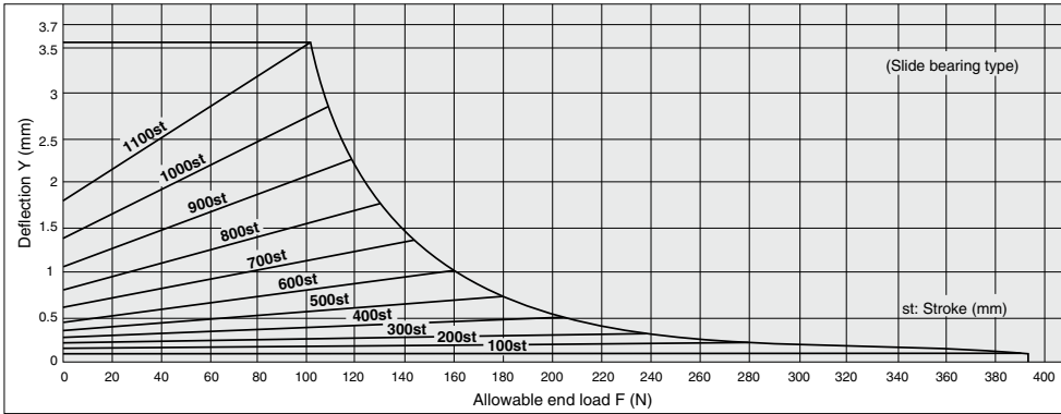
MGGM 63-Stroke
