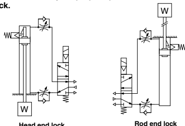
Head end lock
