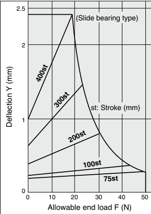
MGG 20-Stroke
