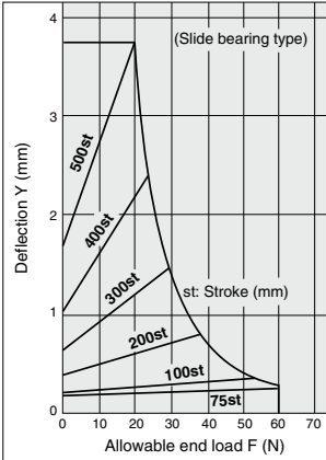
MGG 25-Stroke
