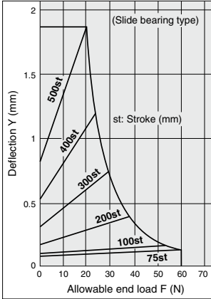
MGG 25-Stroke
