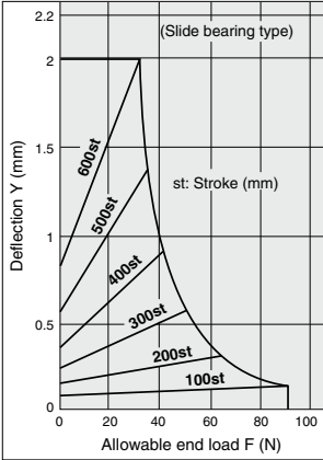
MGG 32-Stroke
