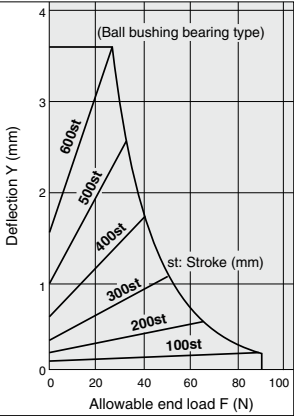
MGGL 32-Stroke
