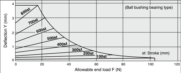
MGGL 40-Stroke
