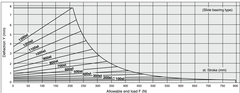
MGGM 100-Stroke
