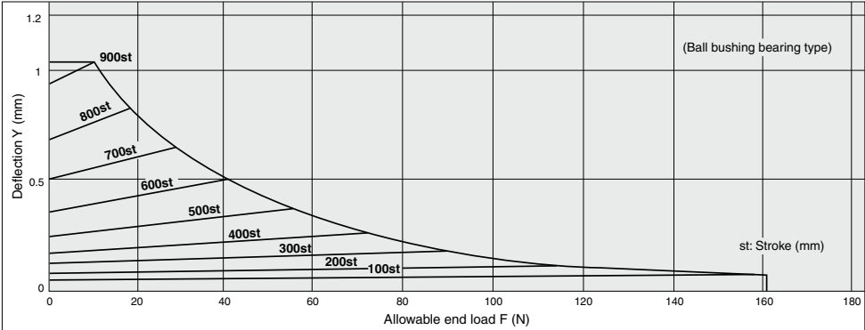
MGGL□63-Stroke
