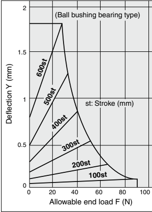
MGGL 32-Stroke
