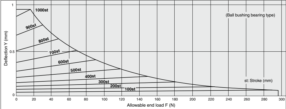
MGGL□100-Stroke
