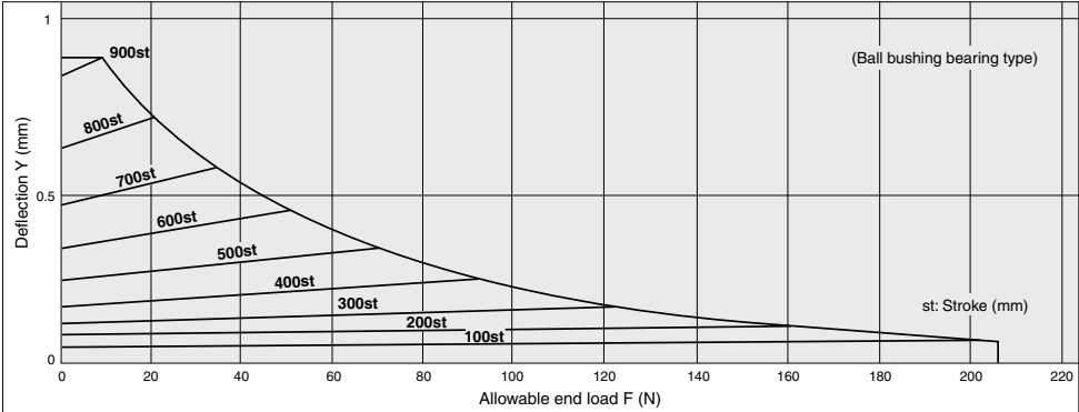
MGGL□80-Stroke
