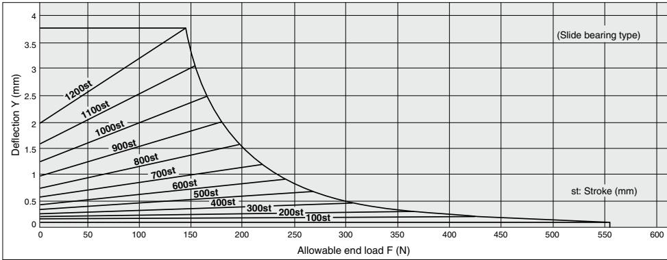
MGGM 80-Stroke
