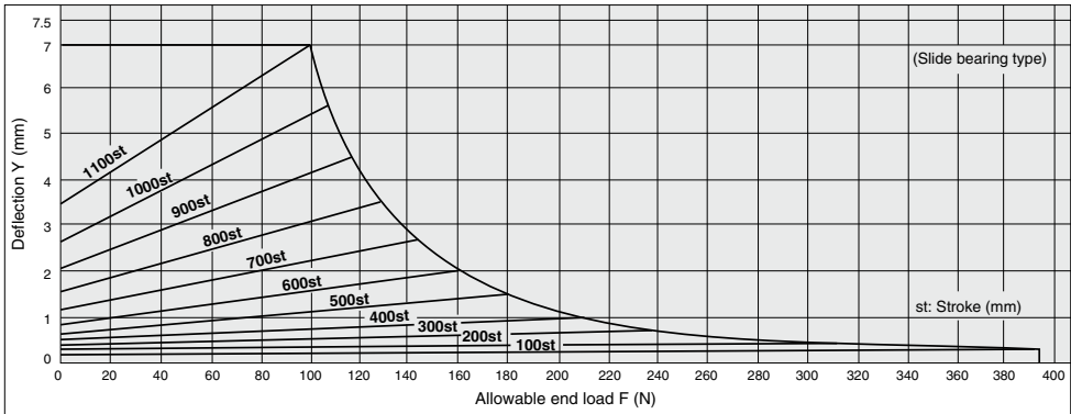
MGGM 63-Stroke
