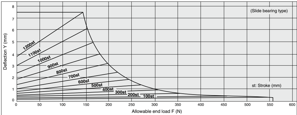
MGGM 80-Stroke
