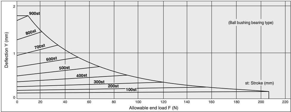
MGGL 80-Stroke
