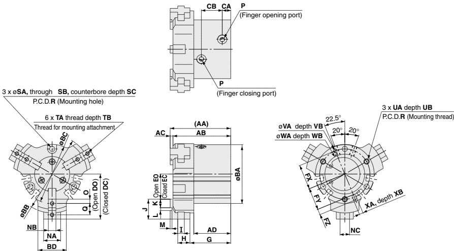
Auto switch mounting groove dimensions (4 locations)
