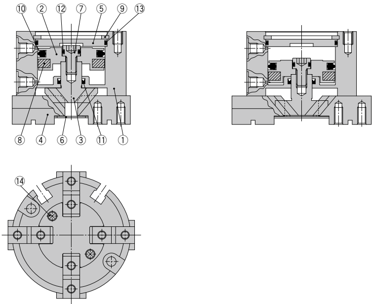
Closed condition
