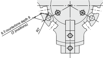
Mounting hole counterbore dimensions MHSL3-32D
