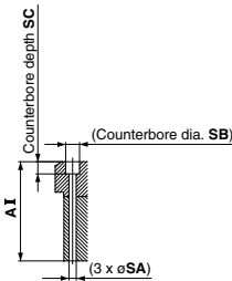
Section SD - SD
