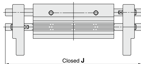
View K (Fingers closed)
