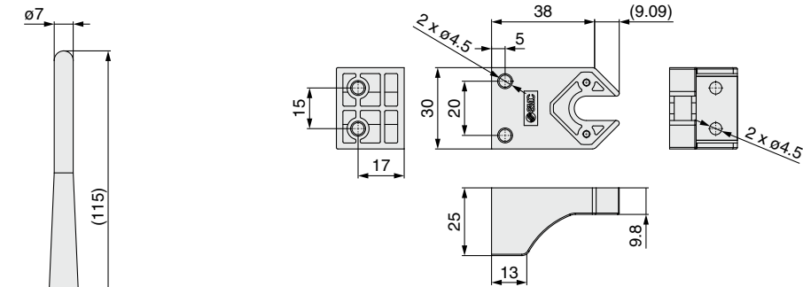
③ Bracket
