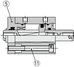
Built-in One-touch fittings
