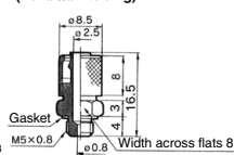
CJ-5H-6 (For ø6/ø4 tubing)
