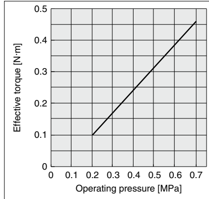
Size 40
