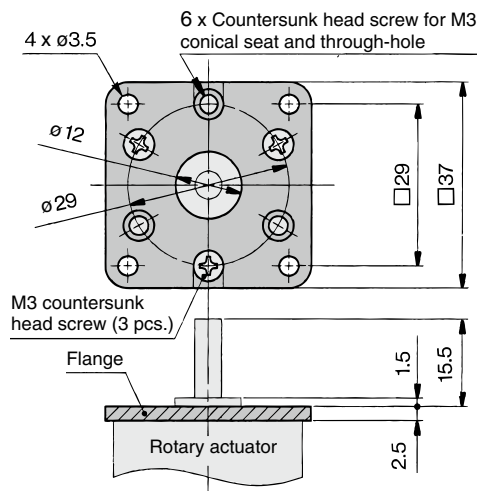
Flange assembly for size 15 Part no.: P211090-2
