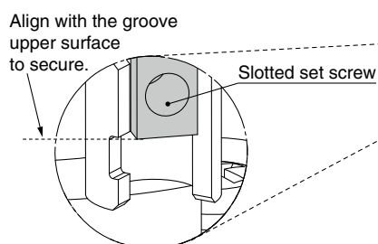
Enlarged view
