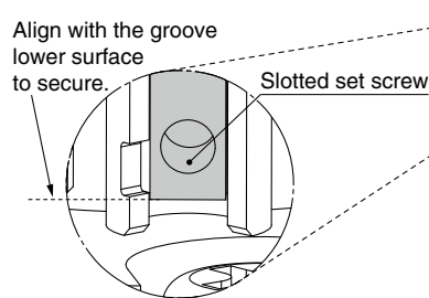
Enlarged view
