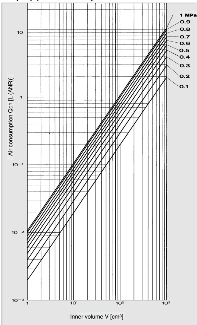
Graph (4) Air Consumption
