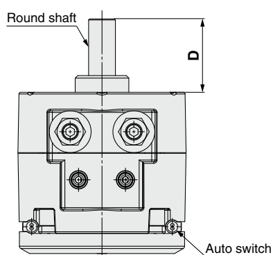
Single shaft/CDRBT□
