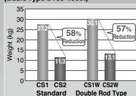
CS1→CS2 Weight Comparison (Basic Type ø160-100st)
