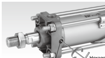
Cushion valve
