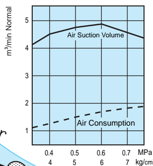
Air Suction Volume and Air Consumption
