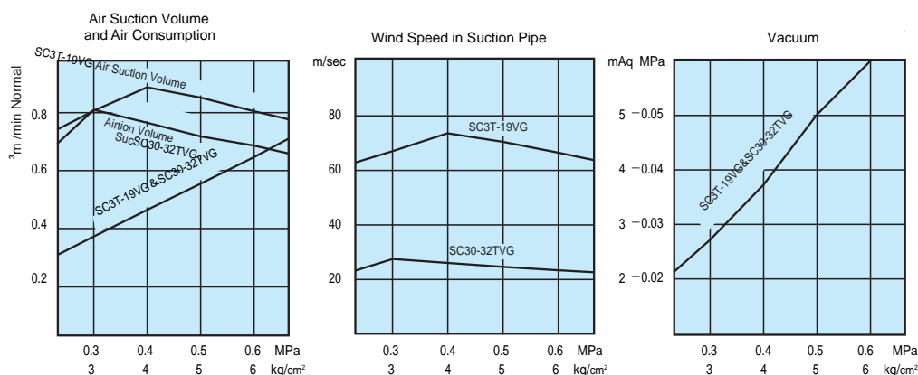
■ Performance Chart (SC30-32TVG)
